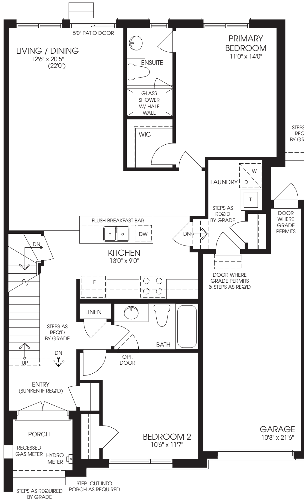
MAIN FLOOR PLAN ELEVATION 'A1'
