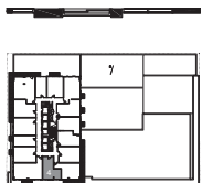
FLOORS 19, 24-27 492 Sq.Ft. French Balcony
