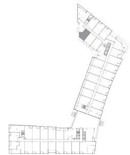
FLOORS 2-7
