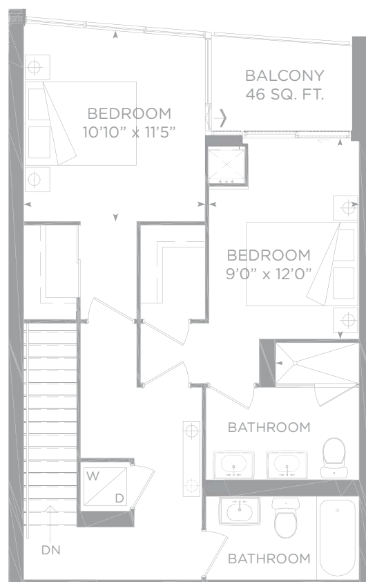
UPPER LEVEL
