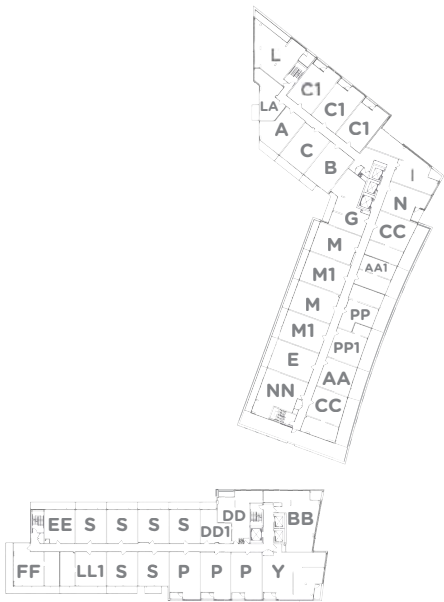
6TH FLOOR
